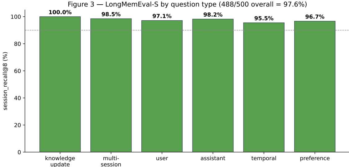
Figure 4: LongMemEval-S session recall@8 by question type (v4 unified 488/500). Preference questions reach 96.7% (29/30) with v4 pref-facts indexing; temporal reasoning is the main remaining gap.
