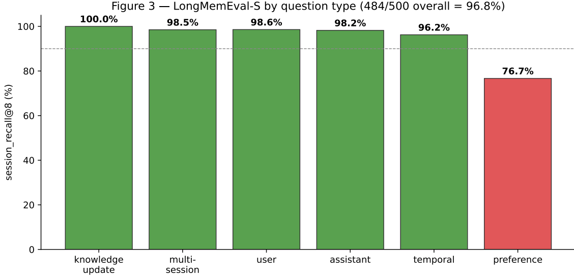
Figure 3: LongMemEval-S session recall@8 by question type. Preference questions (76.7%) remain the main gap—implicit user context not named in the query.
