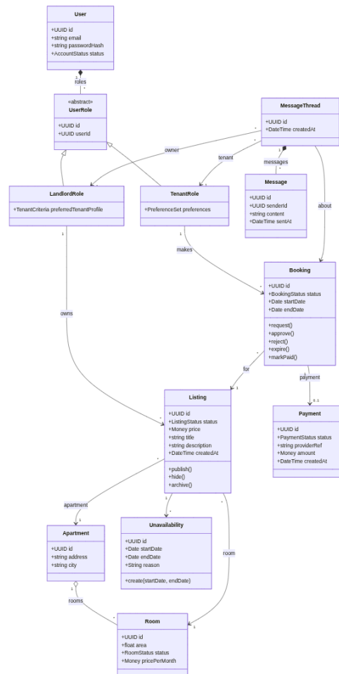
Rysunek 5: Diagram klas - model domenowy (User + Role, Listing, Apartment/Room, Booking, Payment, Messaging)
