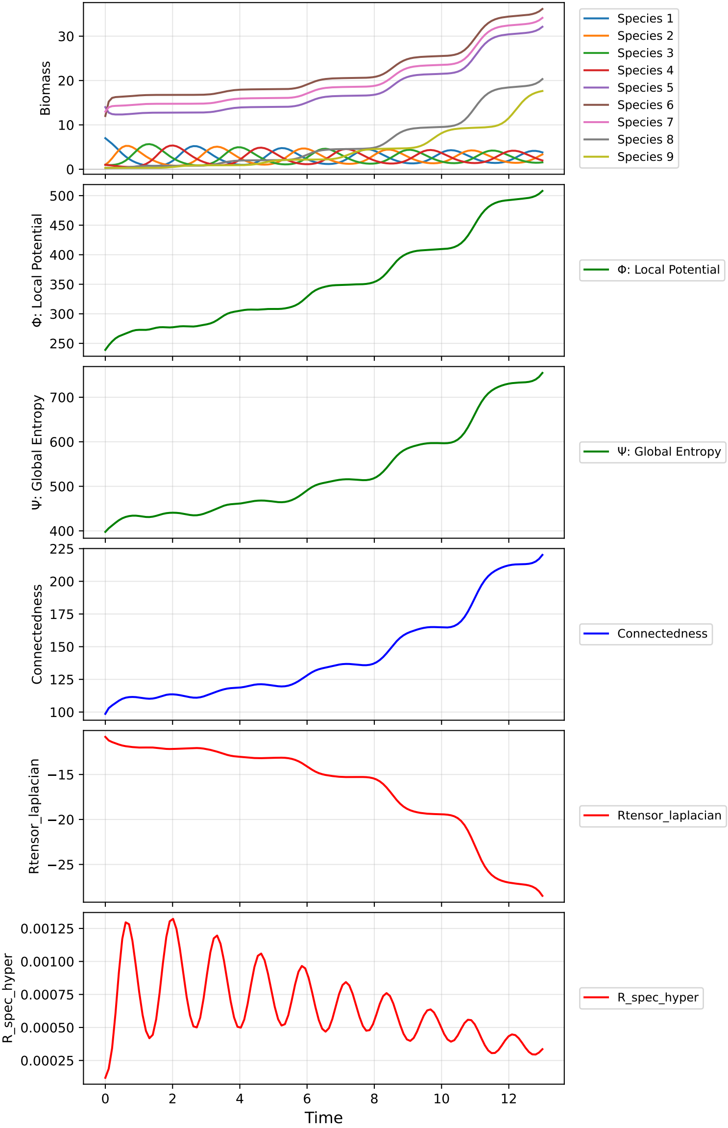
tensor_plots
