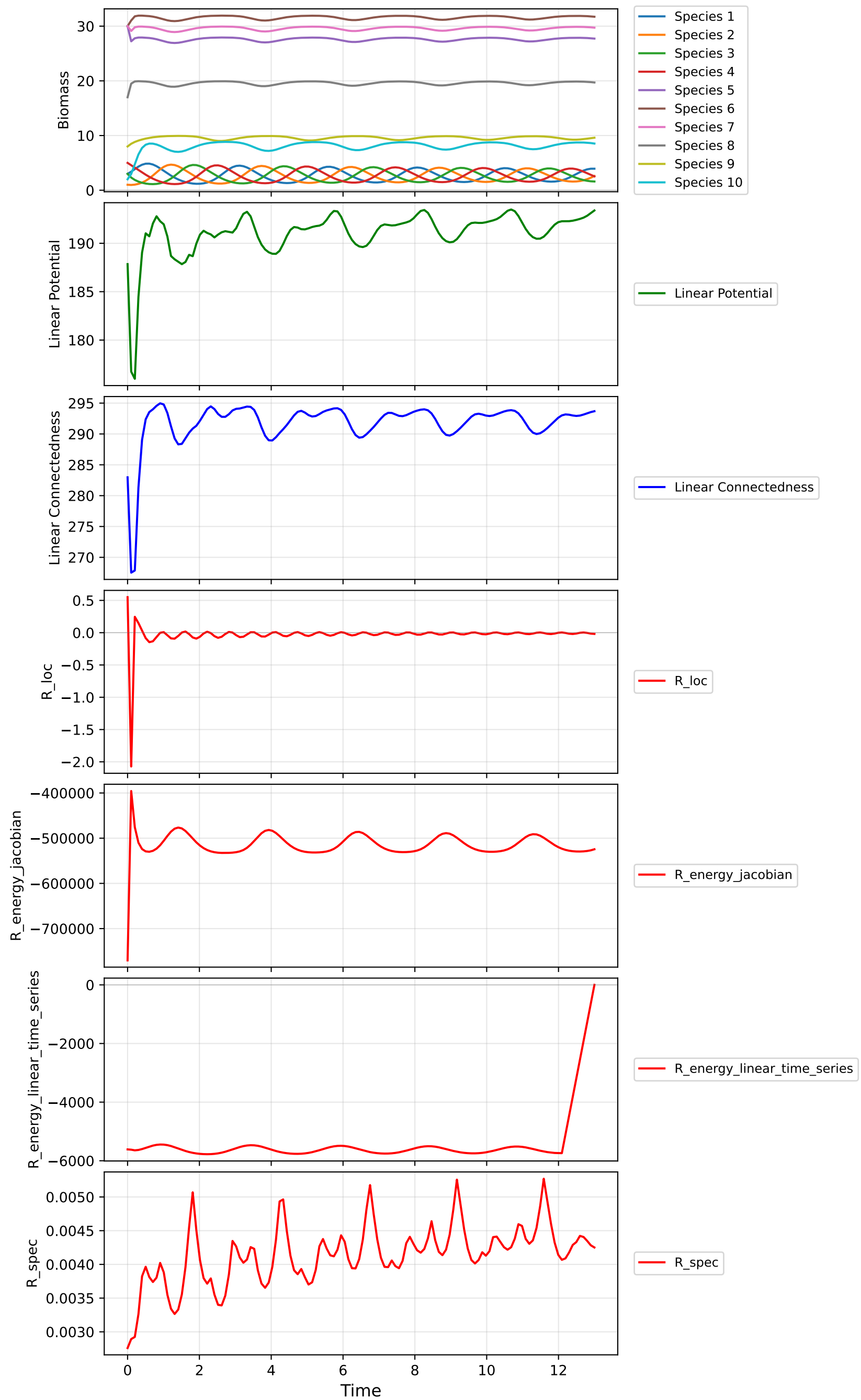
linearized_plots
