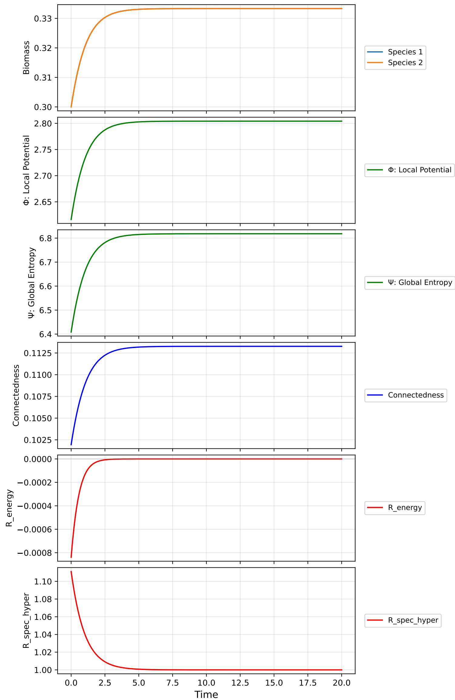
hypergraph_plots
