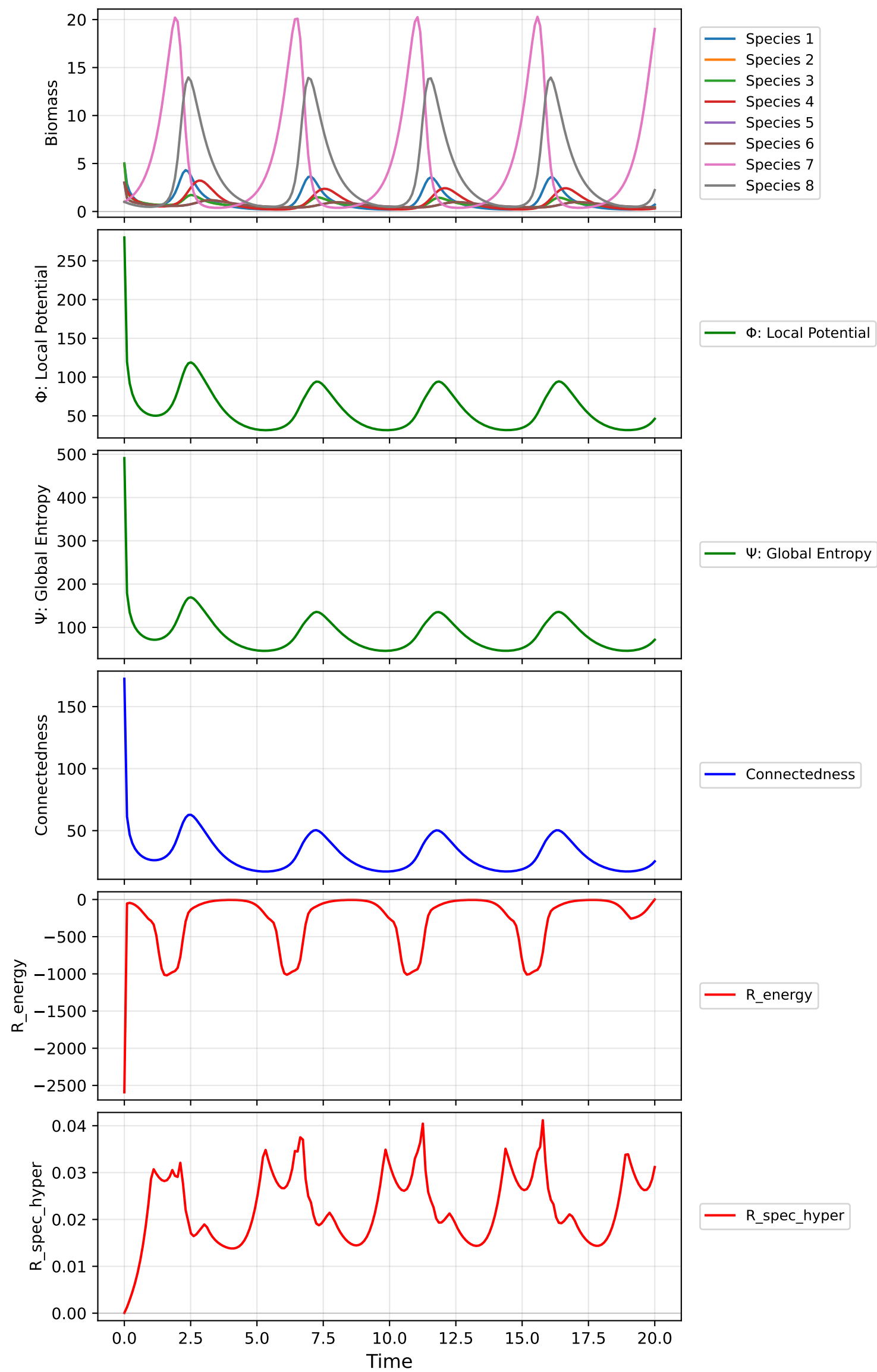
hypergraph_plots
