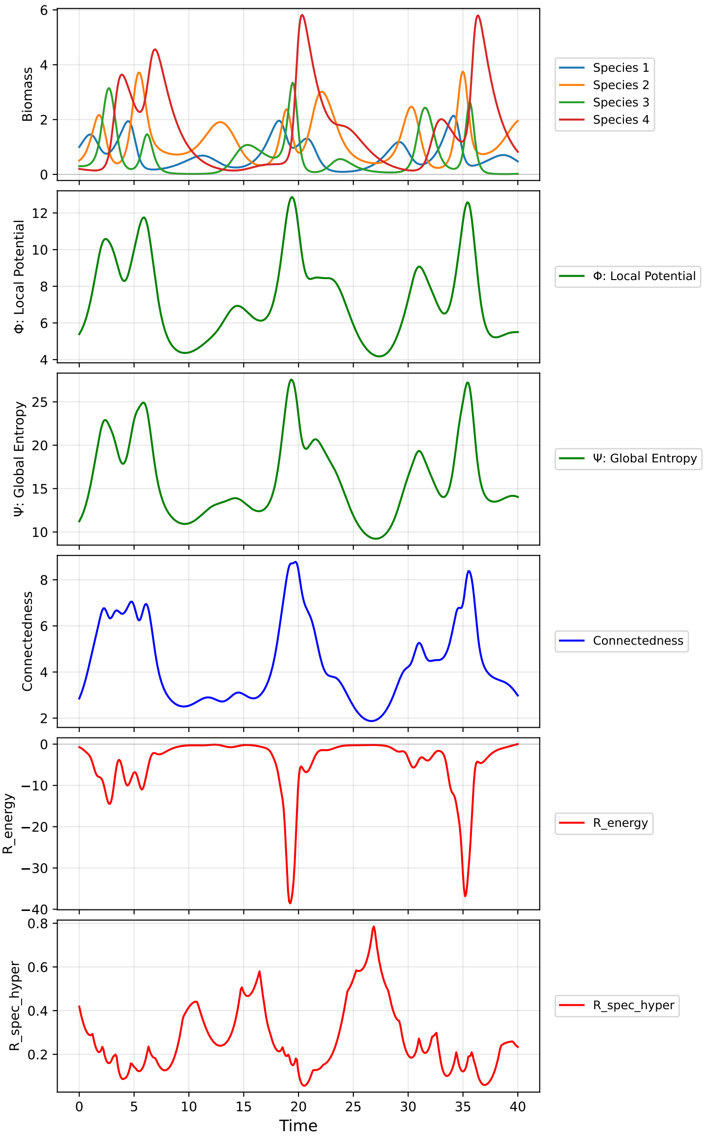
hypergraph_plots
