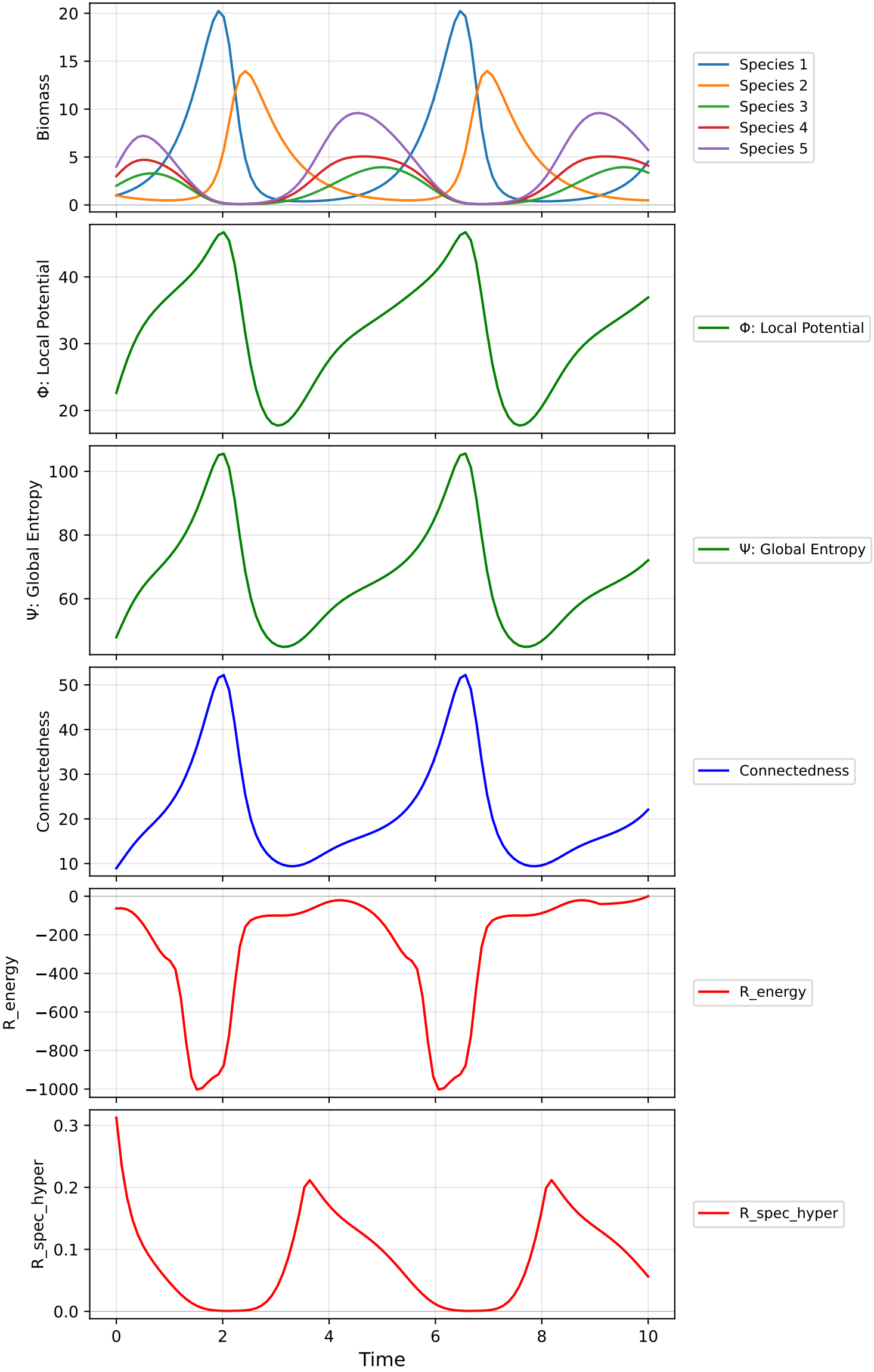
hypergraph_plots
