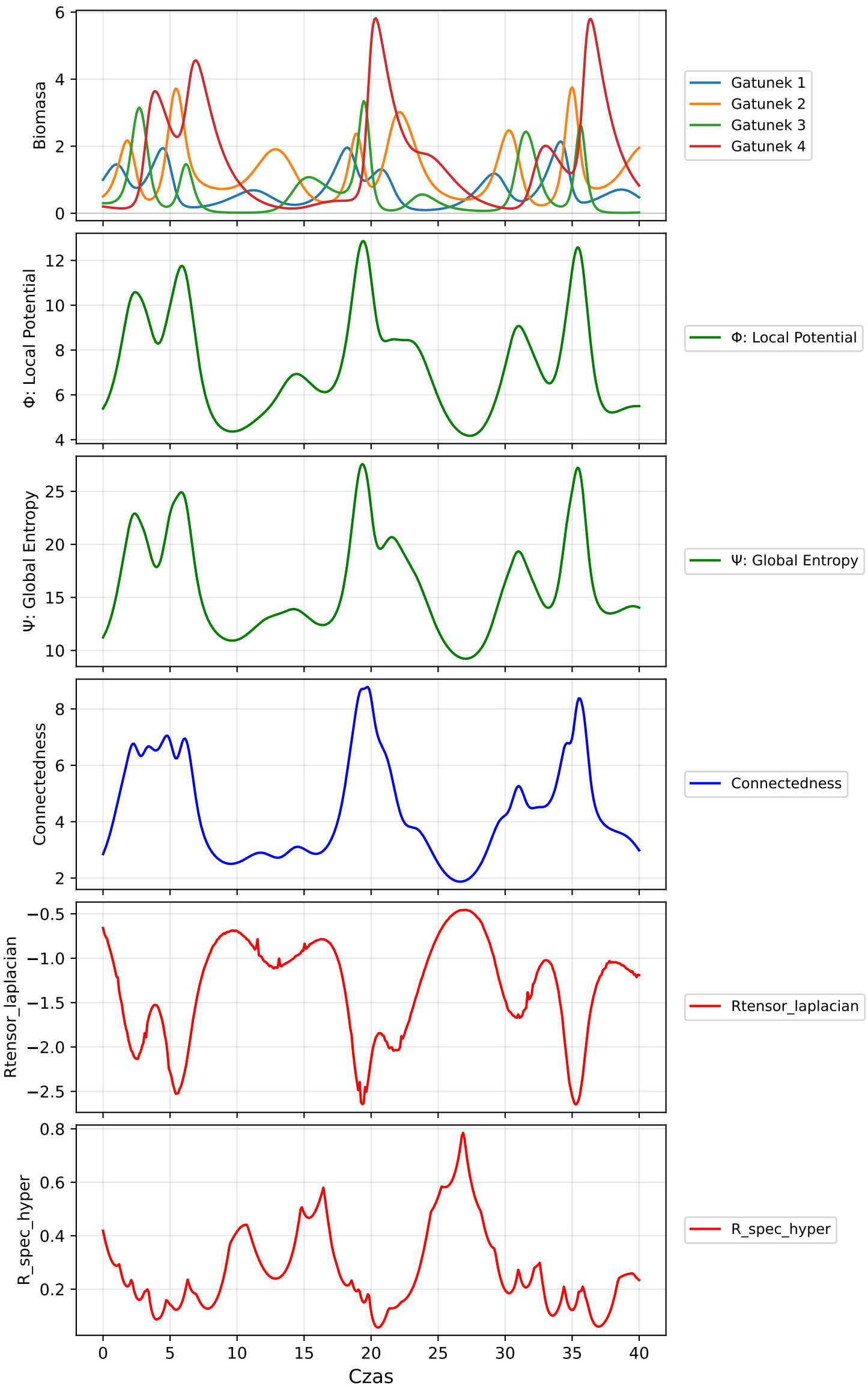
tensor_plots
