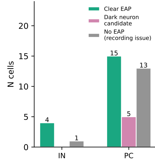
D. EAP on Neuropixels
