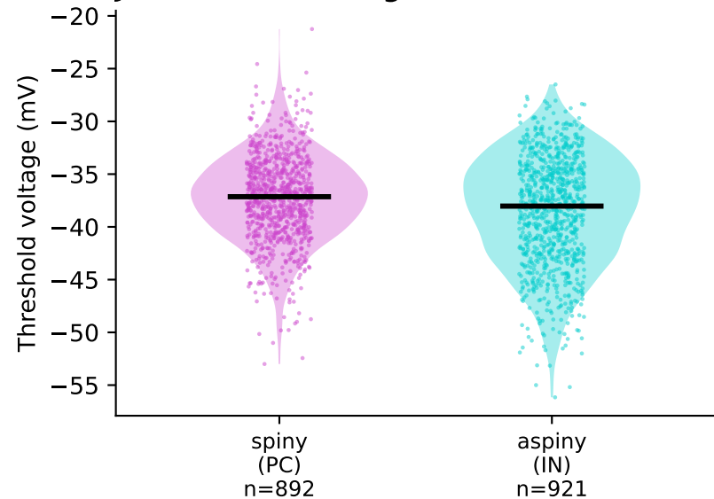
J. Threshold voltage (mV)
