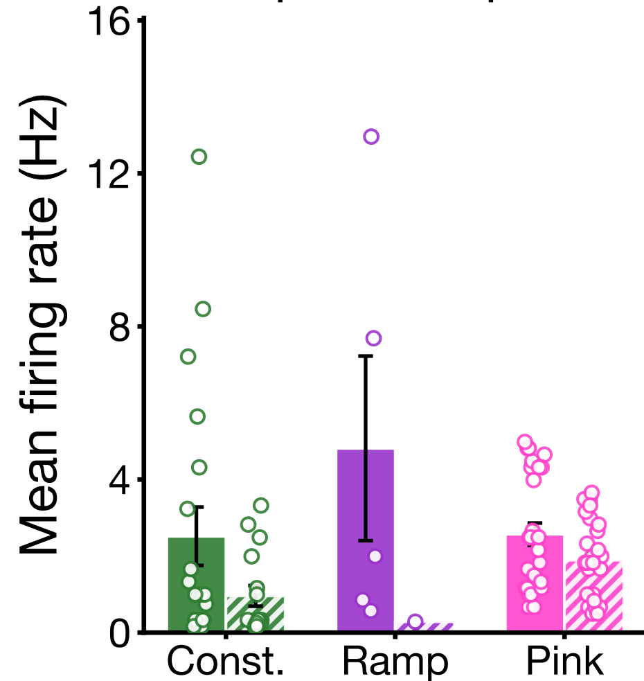
Mean firing rate per sweep
