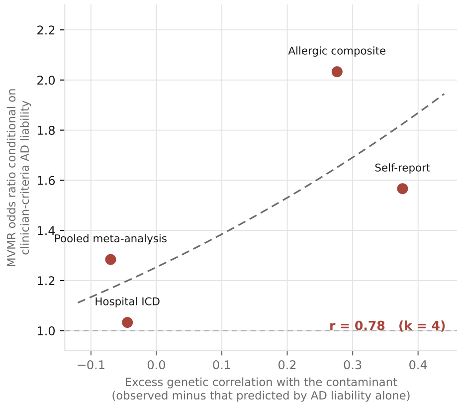
A. The index predicts which definitions are contaminated
