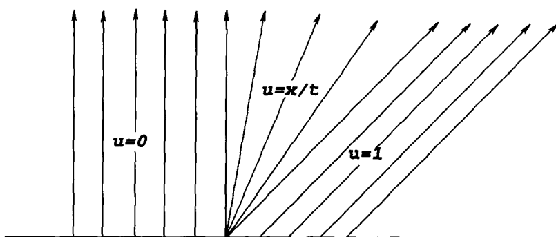
Rarefaction wave
