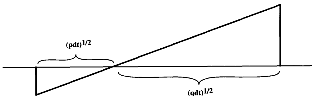
N-wave
