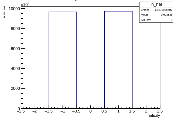
helicity after basic cuts
