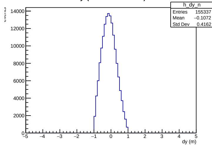
dy (neutron window)
