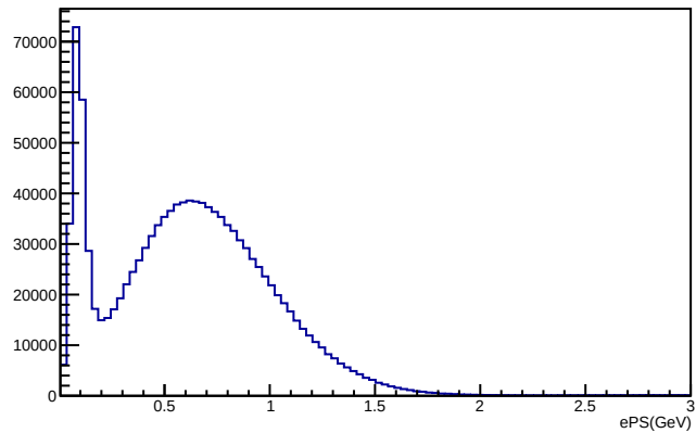
ePS
