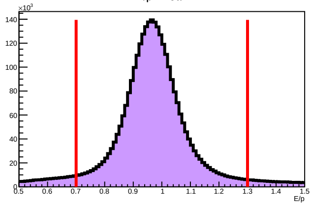
E/p BBCal
