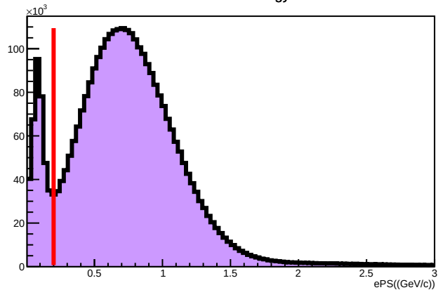
Pre-shower energy
