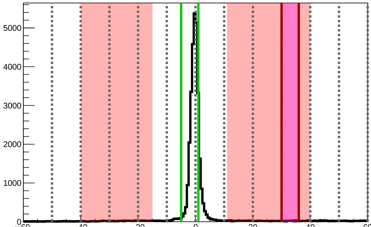
Helicity Asymmetry vs Coincidence time
