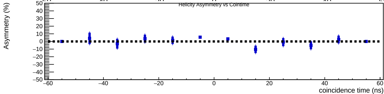
Helicity Asymmetry vs Coincidence time
