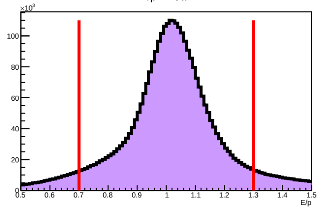
E/p BCal
