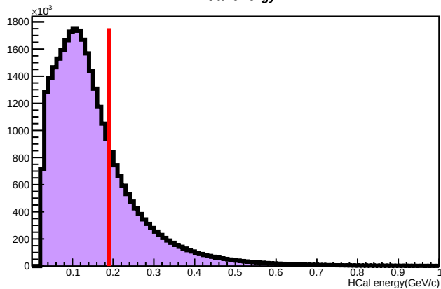
HCal energy
