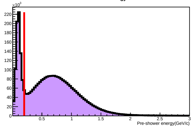
Pre-shower energy
