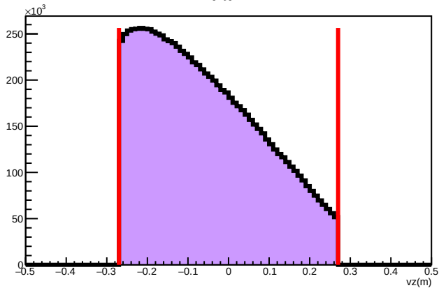
Vertex z
