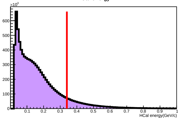
HCal energy
