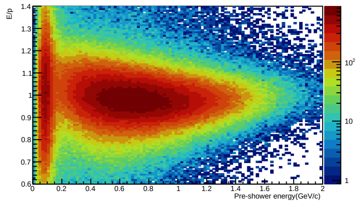
E/p vs Pre-shower energy
