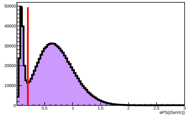
E/p BBCal
