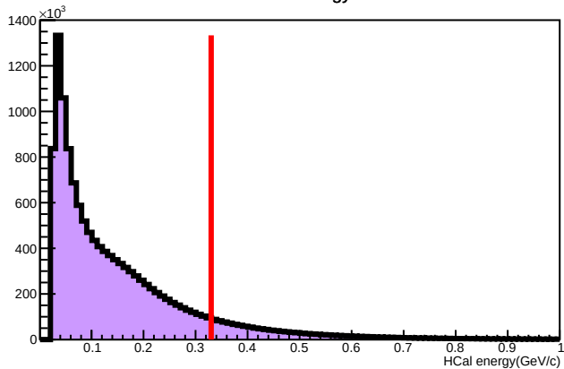
HCal energy
