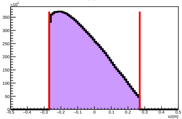
Vertex z
