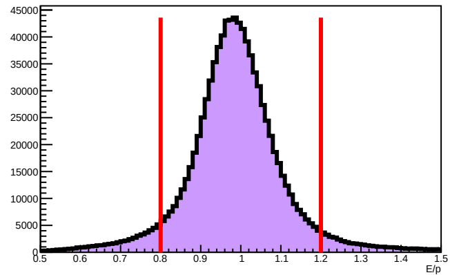
E/p BBCal
