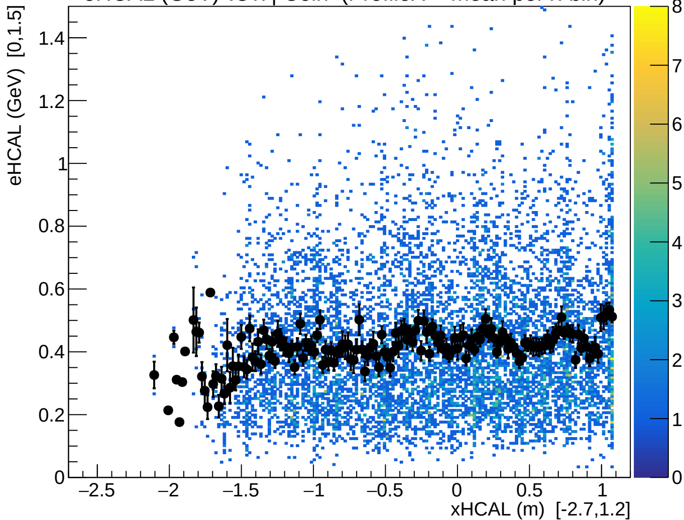
eHCAL (GeV) vs x | Coin (ProfileX = mean per x-bin)
