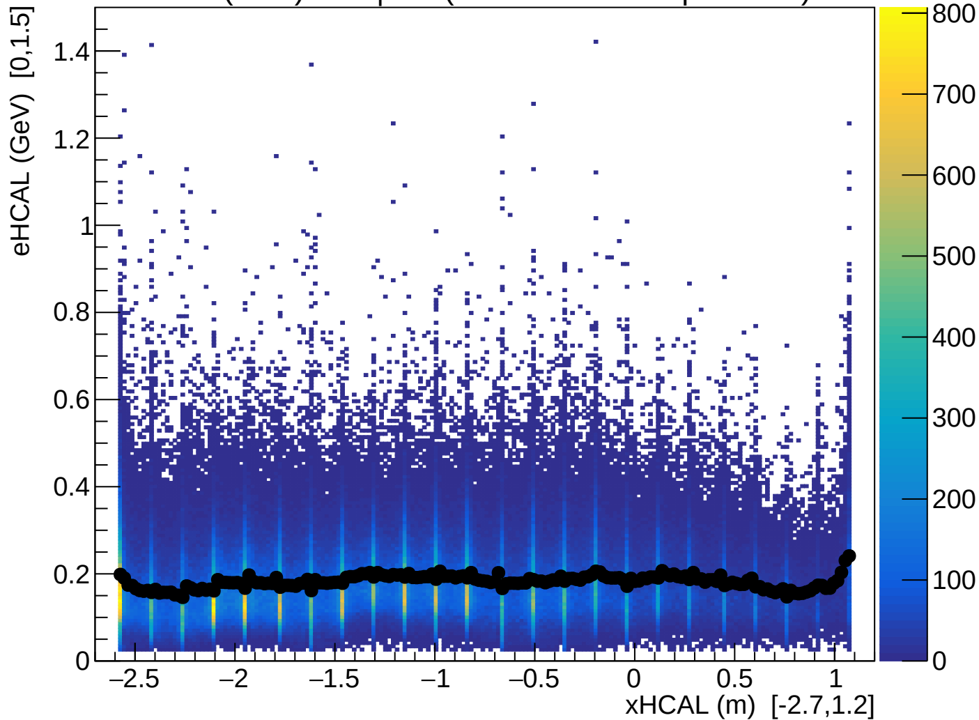
eHCAL (GeV) vs x | All (ProfileX = mean per x-bin)
