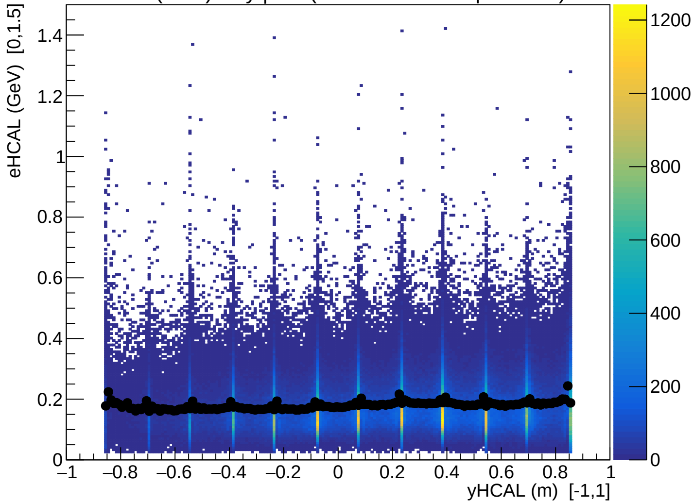
eHCAL (GeV) vs y | All (ProfileX = mean per x-bin)
