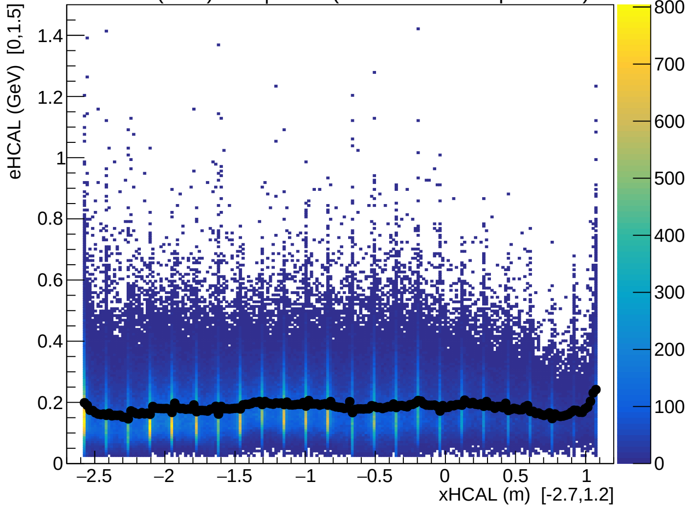
eHCAL (GeV) vs x | Coin (ProfileX = mean per x-bin)
