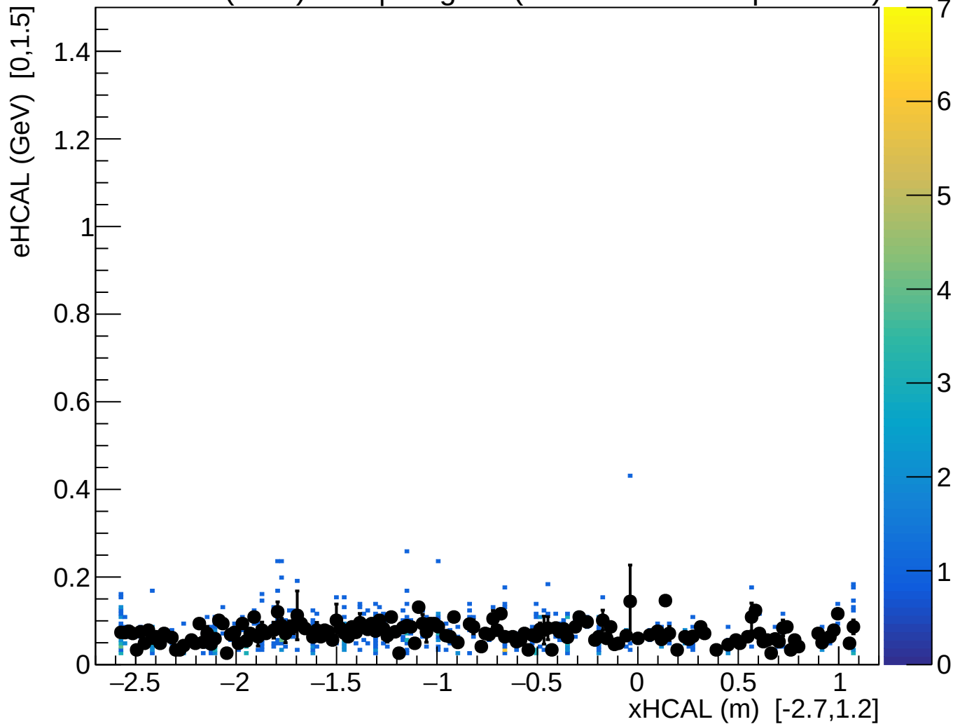
eHCAL (GeV) vs x | Singles (ProfileX = mean per x-bin)
