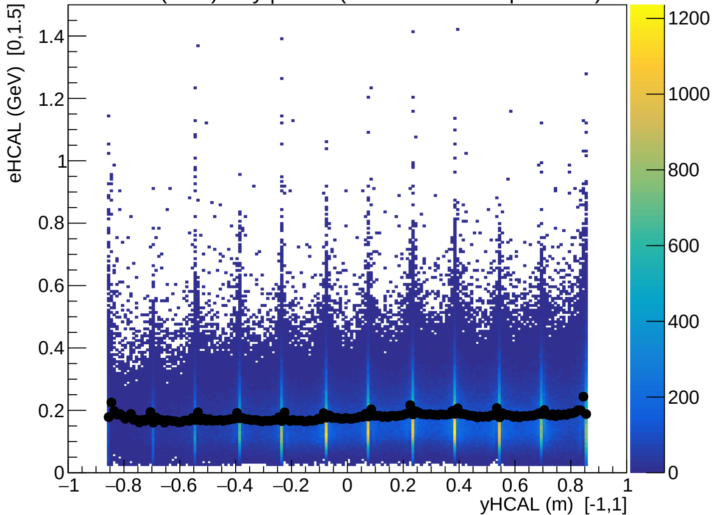
eHCAL (GeV) vs y | Coin (ProfileX = mean per x-bin)
