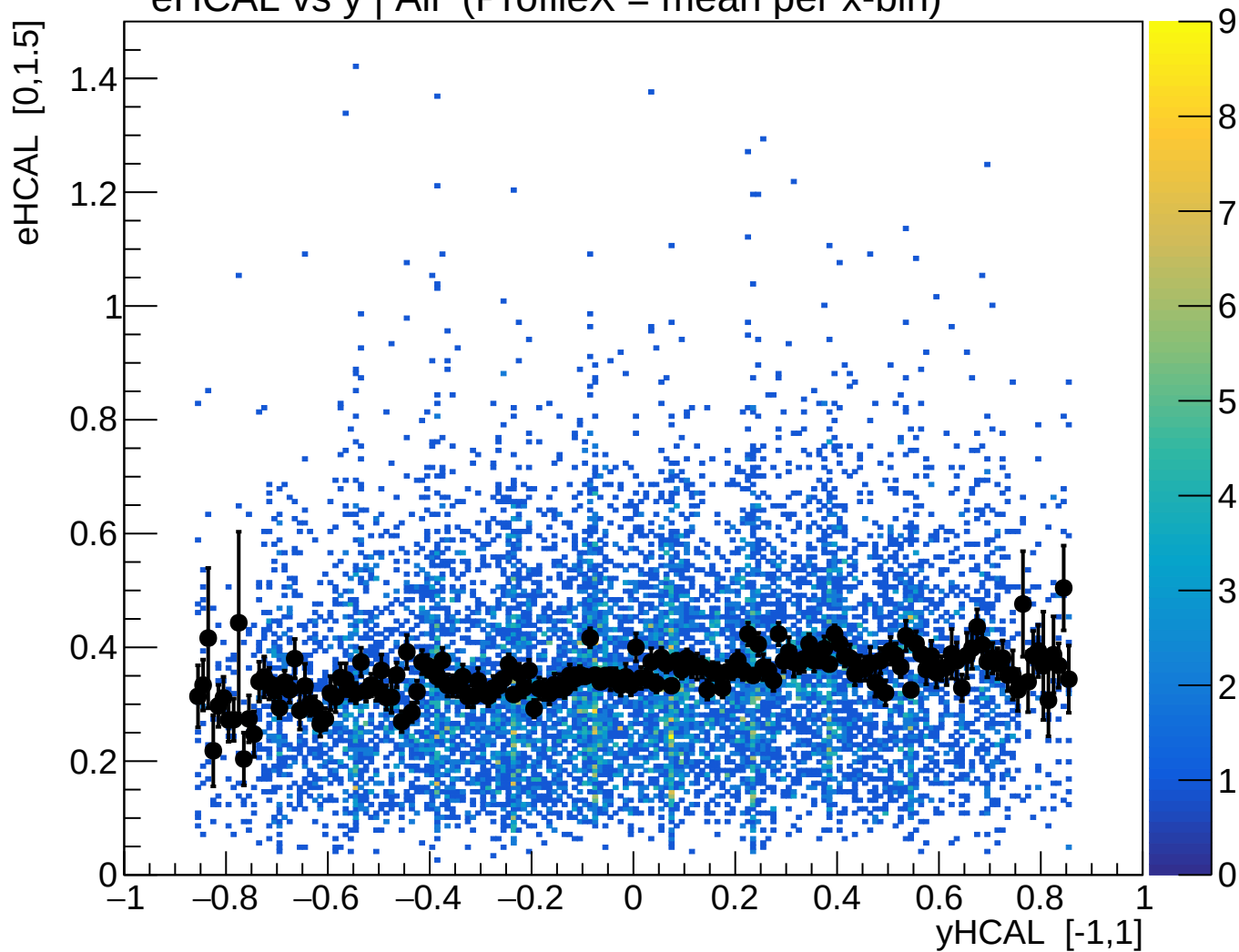
eHCAL vs y | All (ProfileX = mean per x-bin)
