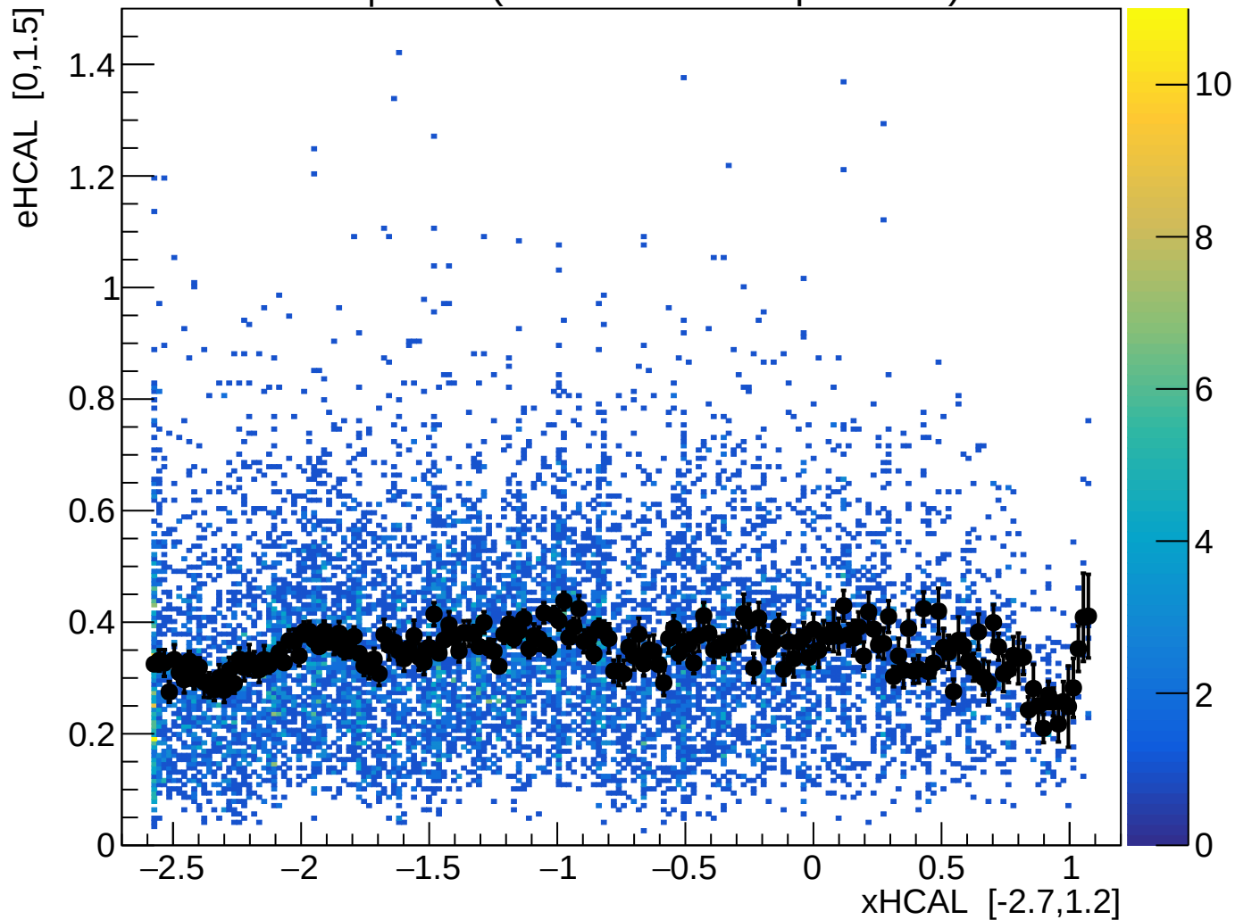
eHCAL vs x | Coin (ProfileX = mean per x-bin)
