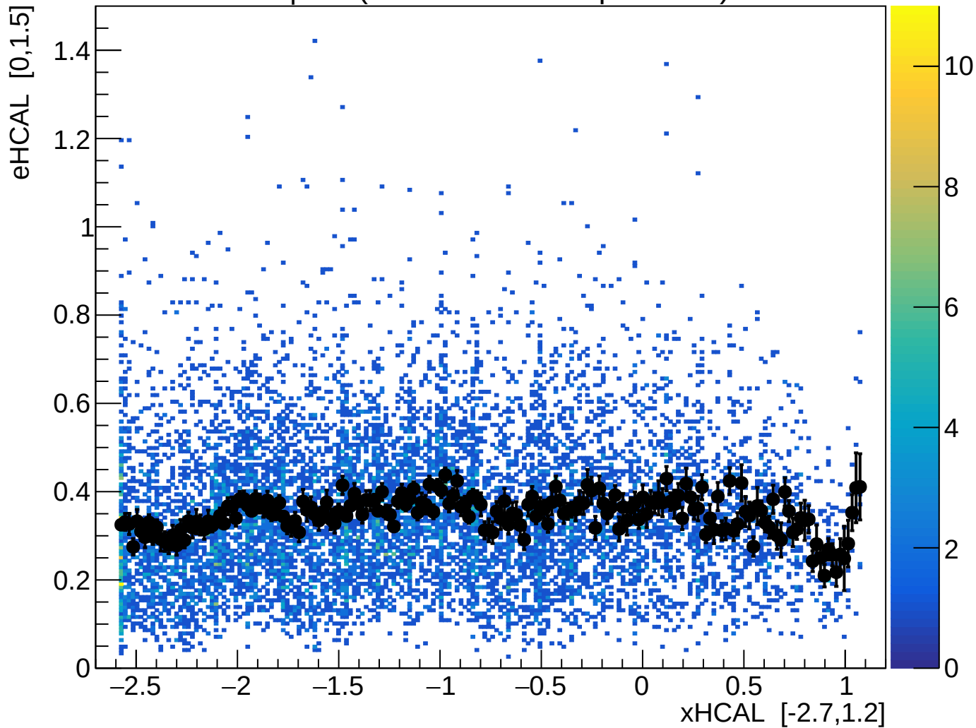
eHCAL vs x | All (ProfileX = mean per x-bin)
