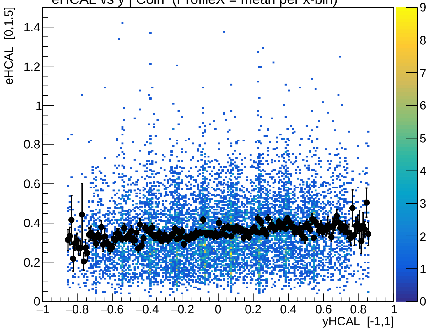
eHCAL vs y | Coin (ProfileX = mean per x-bin)
