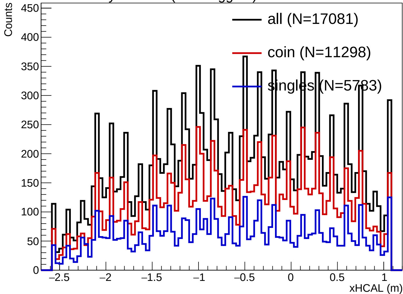
1D overlay: xHCAL (All + triggers)
