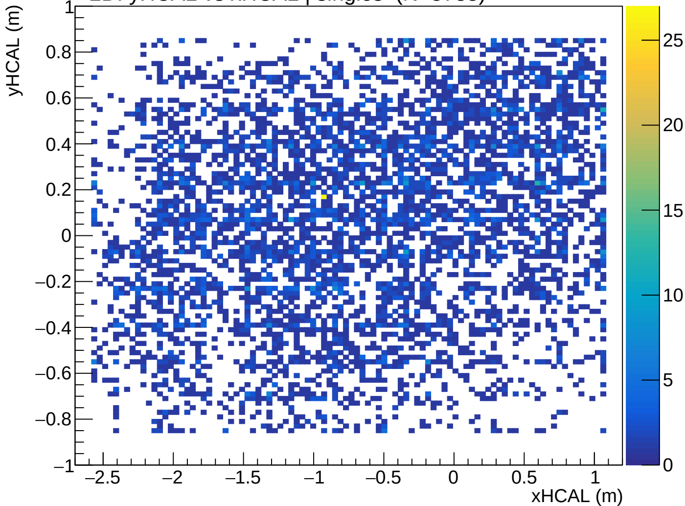
2D: yHCAL vs xHCAL | singles (N=5783)
