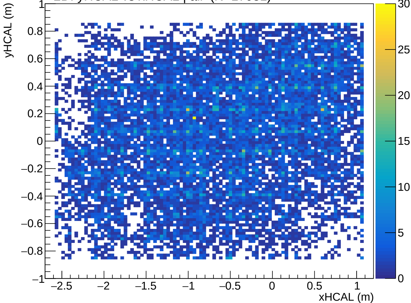
2D: yHCAL vs xHCAL | all (N=17081)
