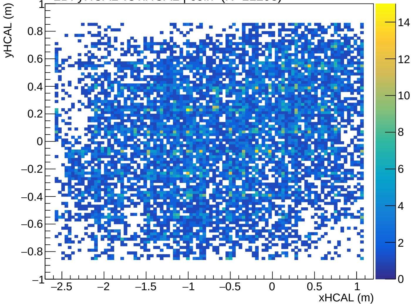
2D: yHCAL vs xHCAL | coin (N=11298)
