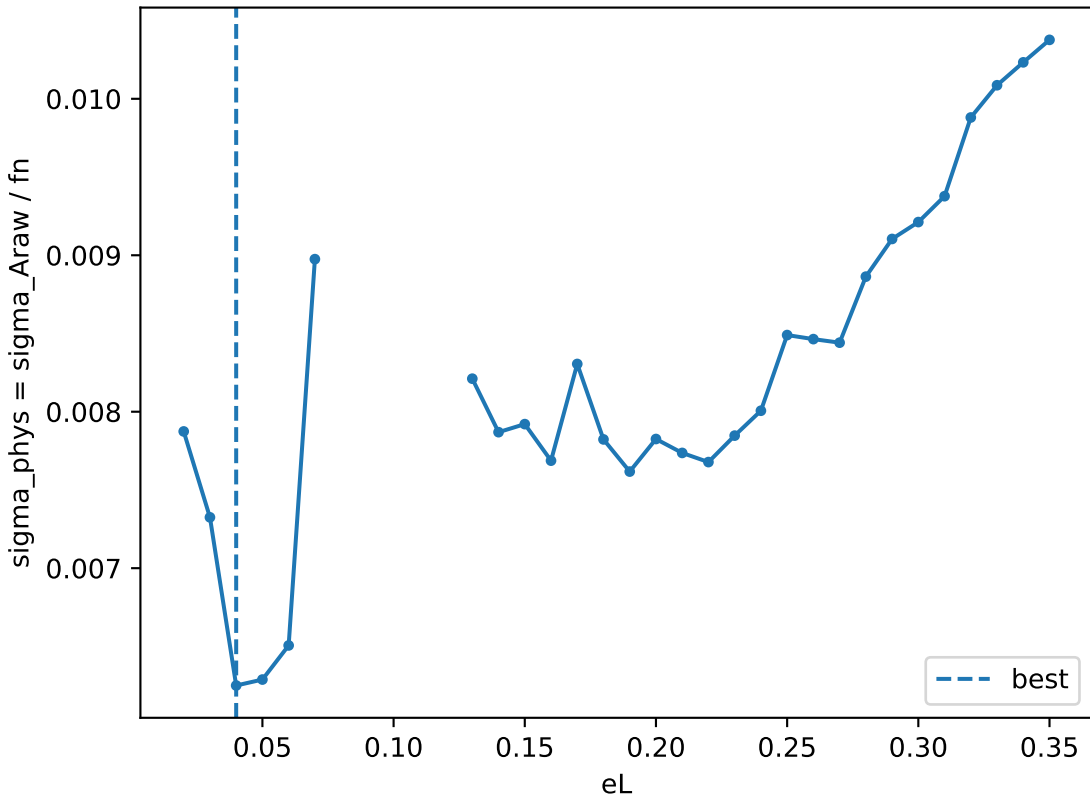
1D scan: eL (others fixed)
