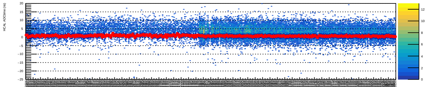
HCAL ADC time vs Run no.
