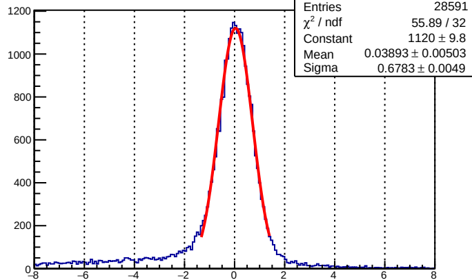
TH - SH ADC Time (ns)
