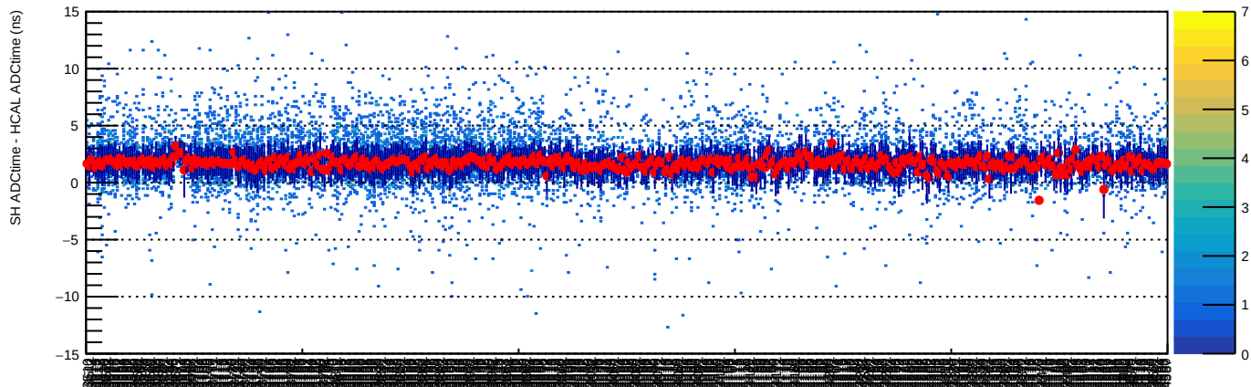
PS-HCAL Coin vs Run No.
