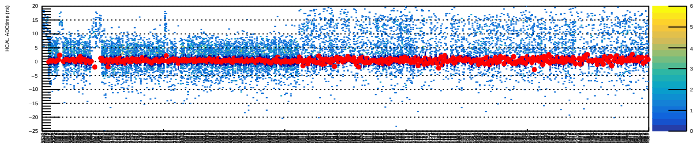
HCAL ADC time vs Run no.
