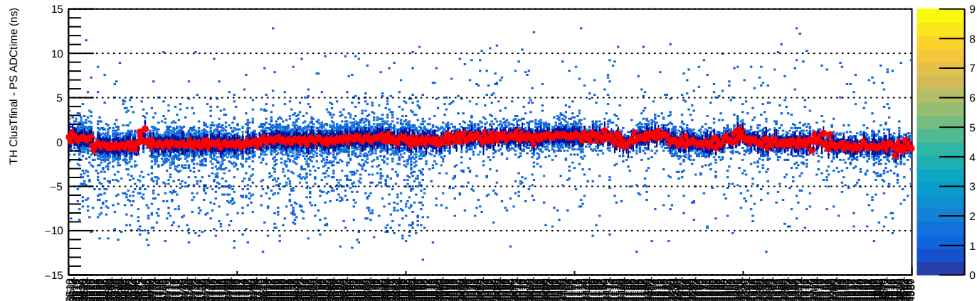
TH-PS Coin vs Run No.
