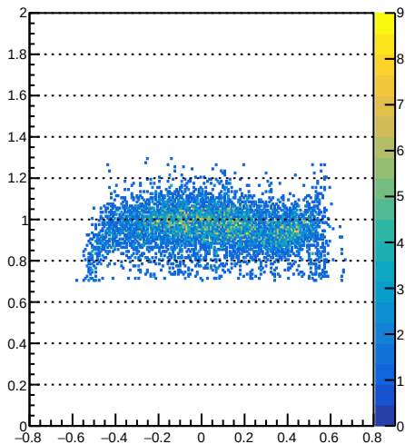
E/p vs Track x
