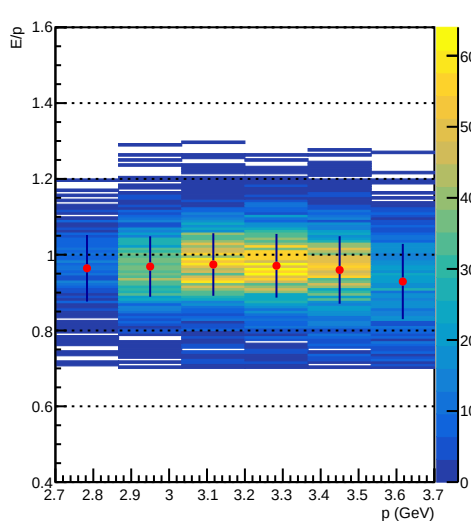
E/p vs p
