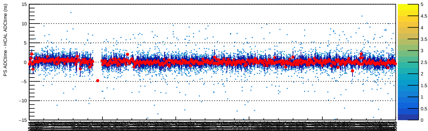
PS-HCAL Coin vs Run No.
