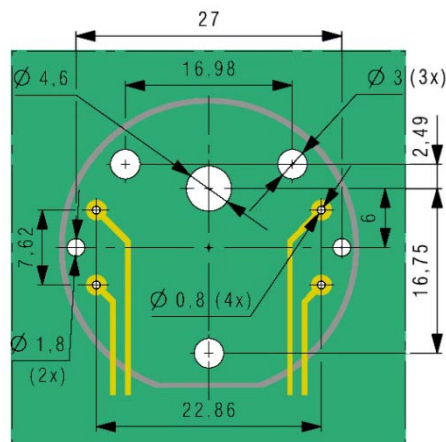
Figure 6: PCB Layout
