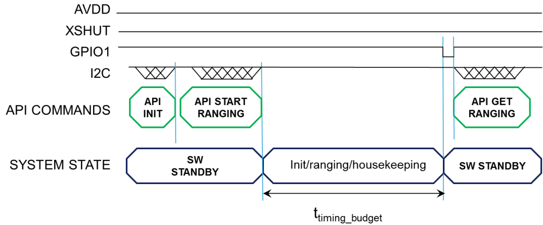
Figure 8. Ranging sequence
