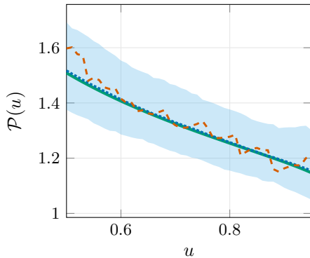
Weibull ( k = 2 )
