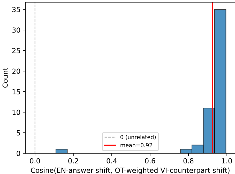
Common-mode shift across 50 answer tokens
