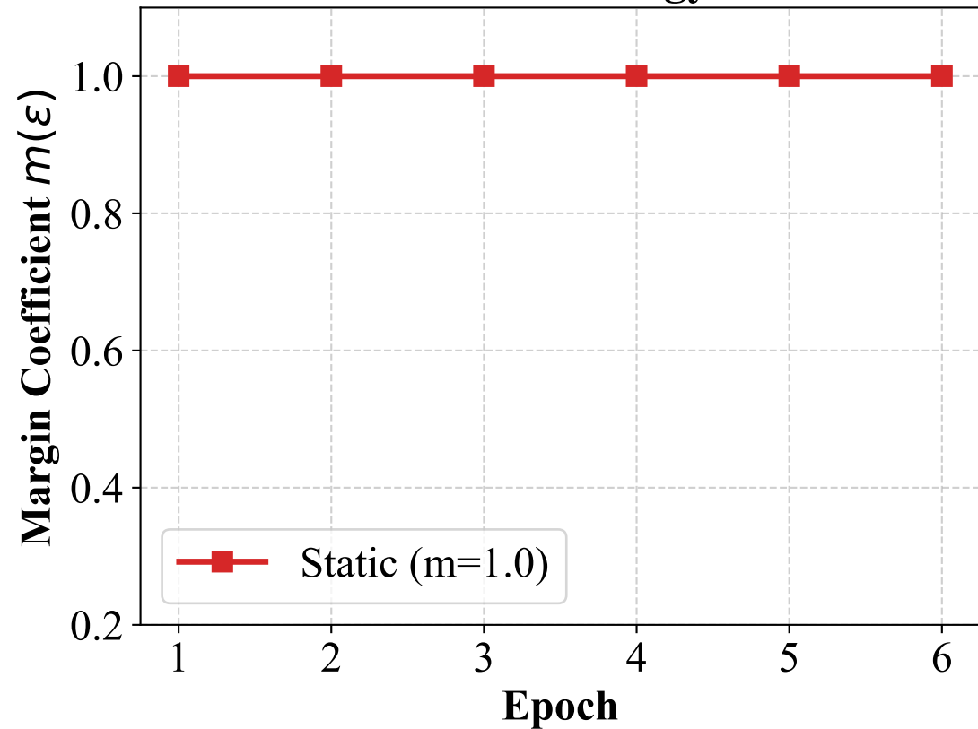
Static Strategy
