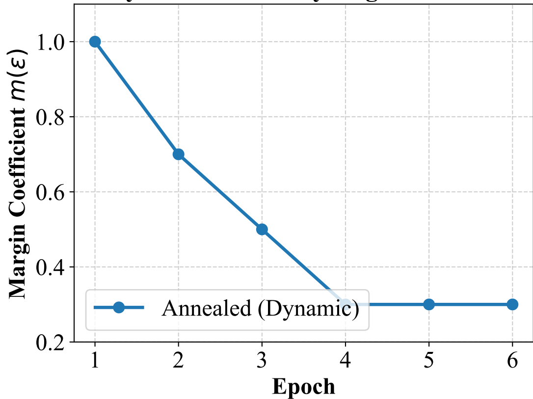
Dynamic Boundary-Regularization
