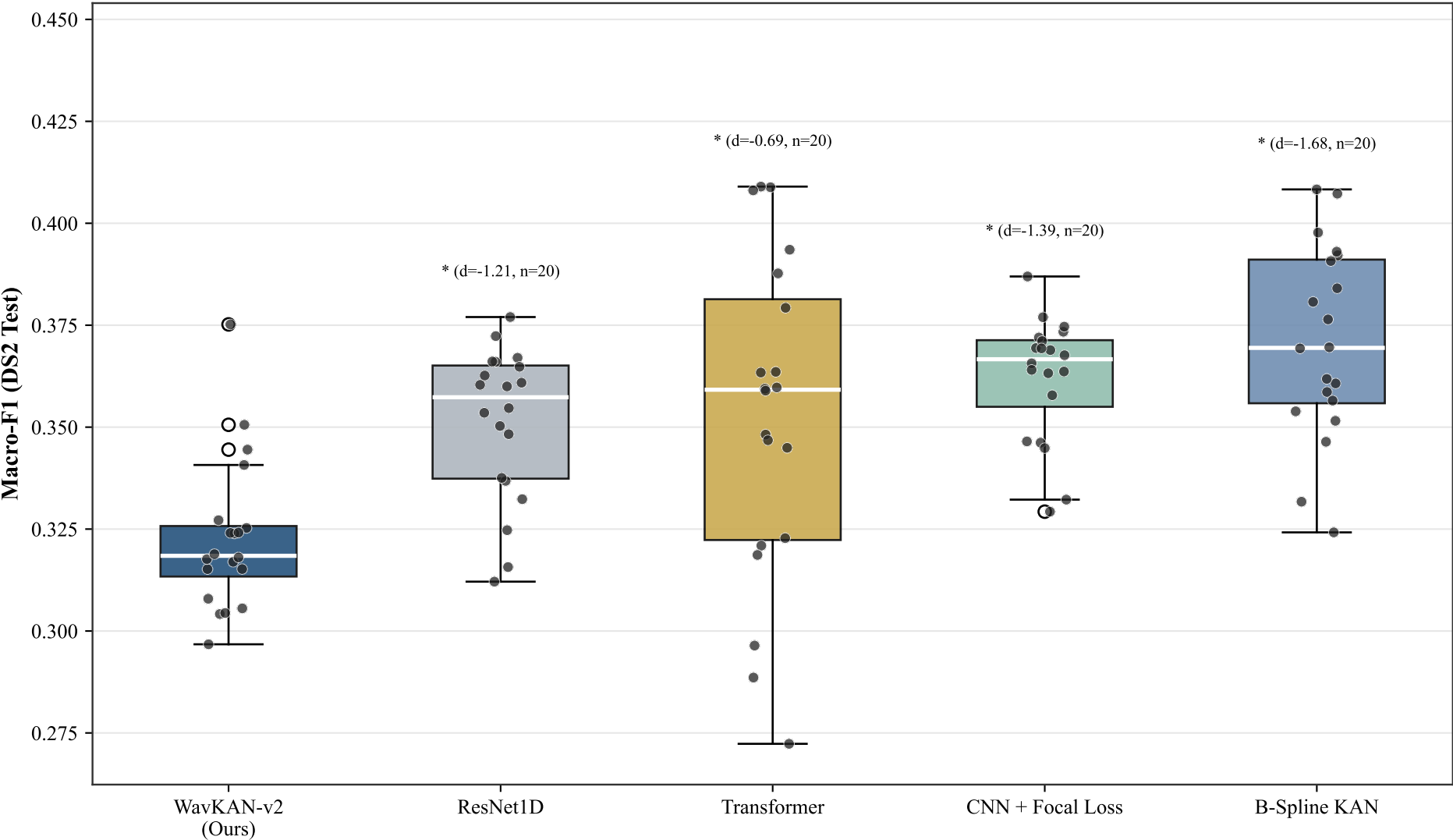
Seed Stability Analysis --- WavKAN-v2 vs. 4 Baselines (real per-seed data; * = Holm-significant, ns = not significant after correction, two-sided Wilcoxon vs. WavKAN-v2, paired by seed identity)
