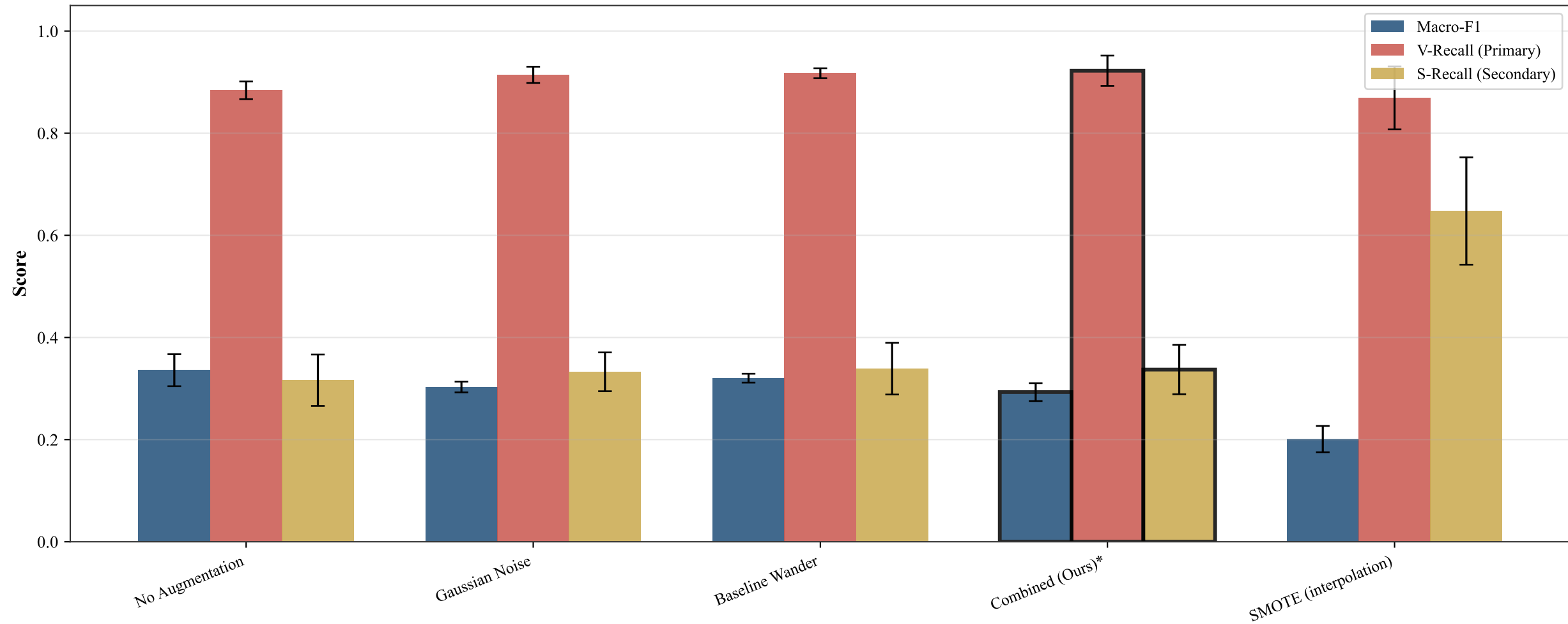
Augmentation Strategy Comparison --- WavKAN-v2 on MIT-BIH DS2 Final (Plain-MLP RR Fusion), 153,045 Params Configuration; * Combined (Gaussian + Wander) is the strategy selected in train_pca.py
