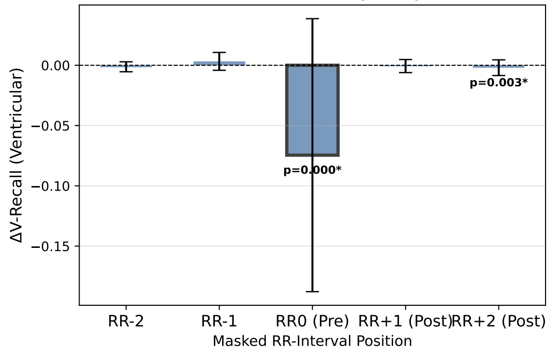
V-Class (Ventricular): sensitivity to rhythm context
