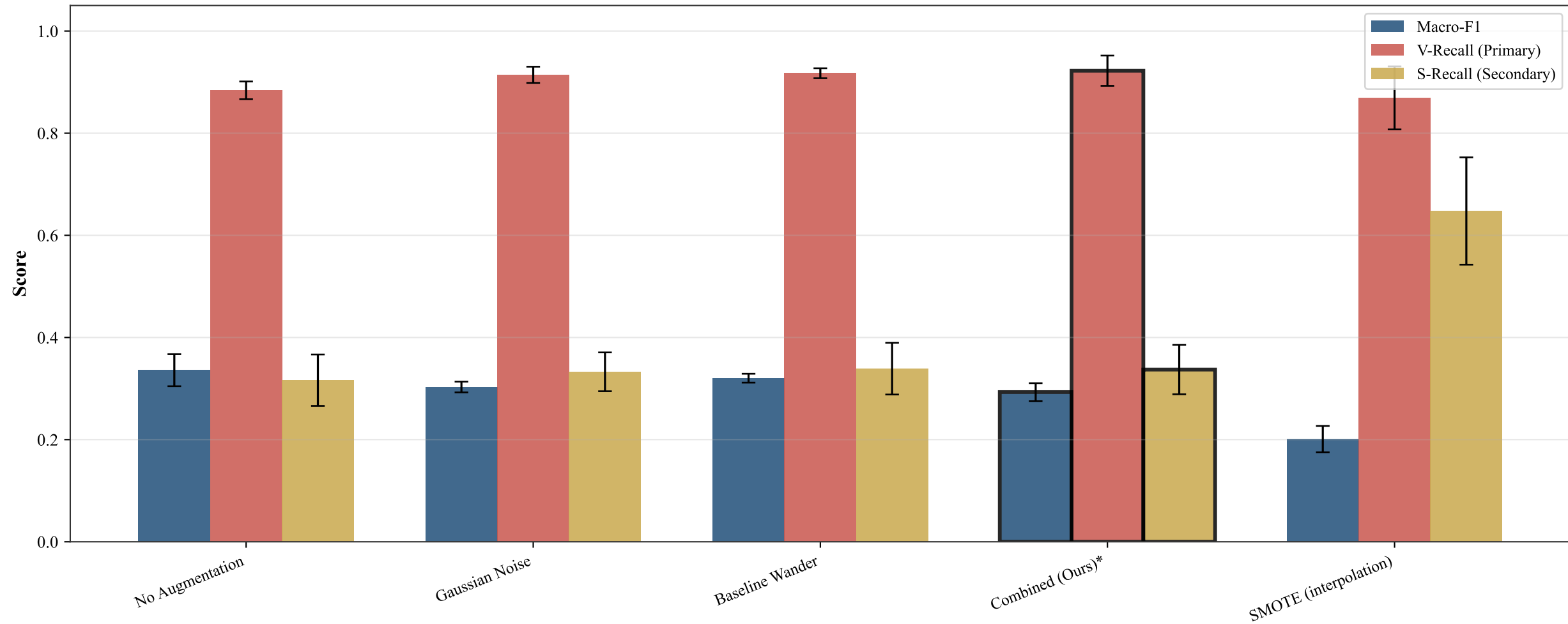
Augmentation strategy comparison --- PC-WavKAN, MIT-BIH DS2 MLP rhythm encoder, 153,045 params; * marks the strategy used in the headline training recipe
