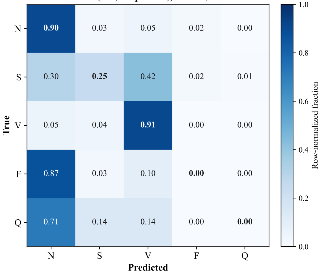
Normalized Confusion Matrix PC-WavKAN (153,045 params), seed 42, DS2 test set
