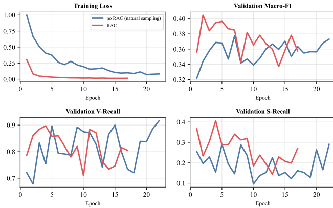
Fig. 4. Per-epoch training dynamics, no-RAC vs. RAC arm (seed 42, DS1 validation Macro-F1), on the base configuration used for the replication in §V-C.
