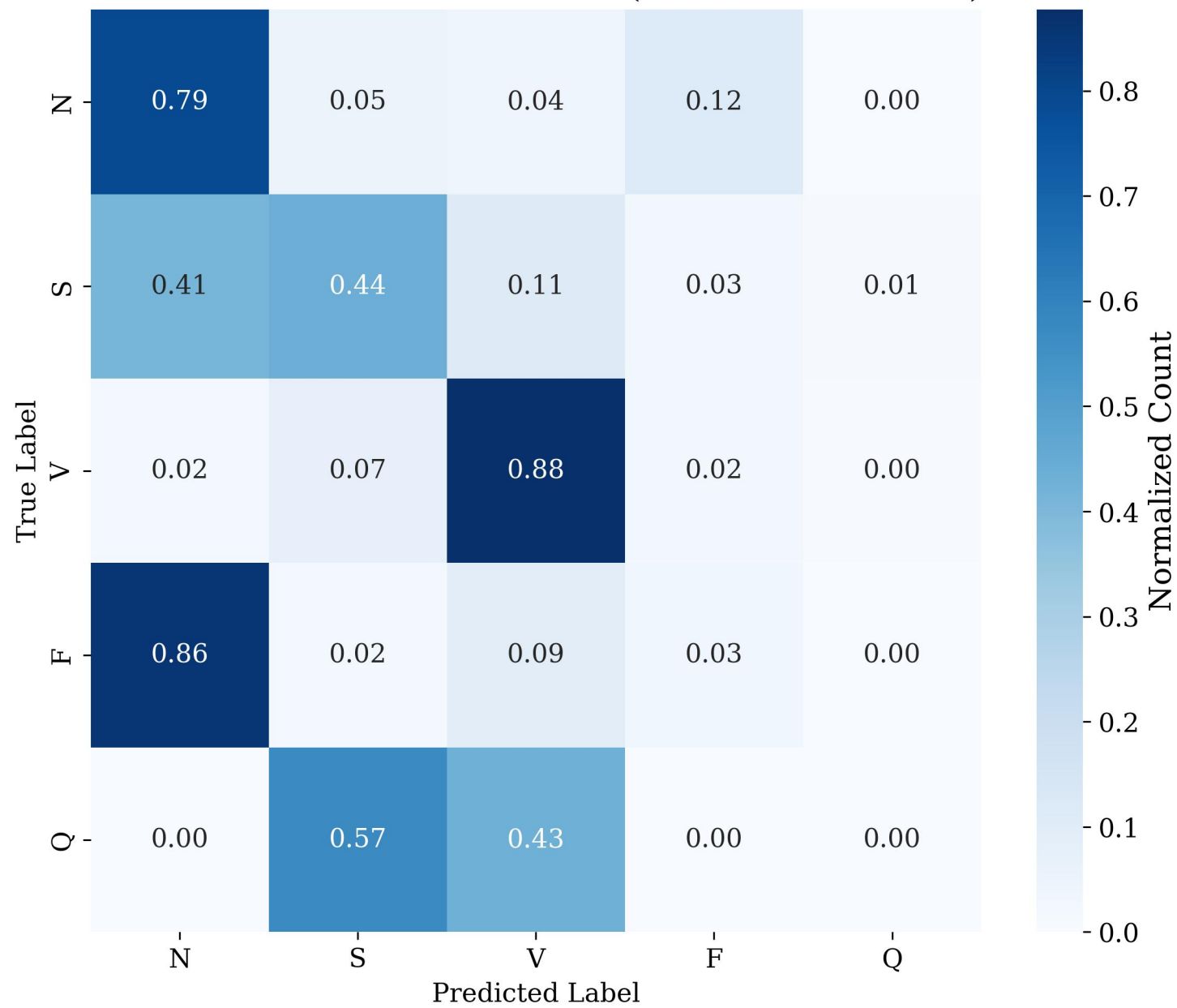
Confusion Matrix on MIT-BIH DS2 (Inter-Patient Test Set)
