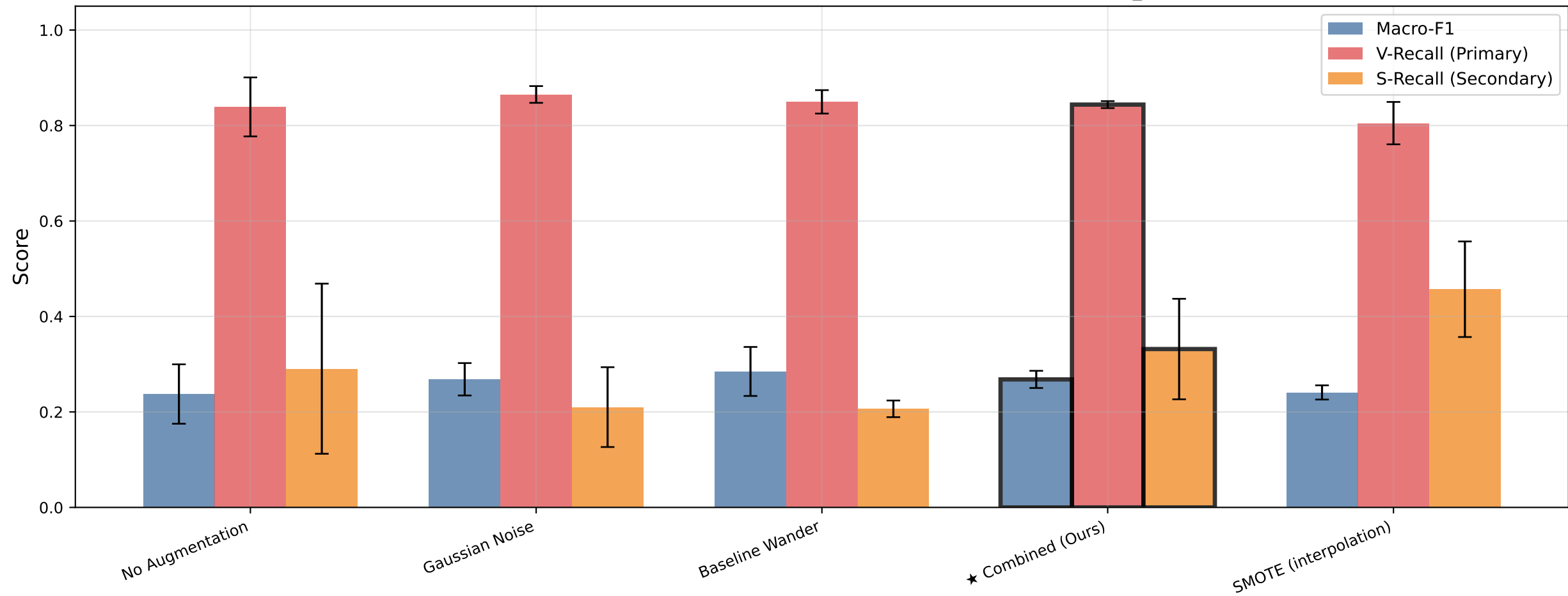
Augmentation Strategy Comparison — WavKAN-v2 on MIT-BIH DS2 ★ Combined (Gaussian + Wander) is our selected strategy in train_pca.py
