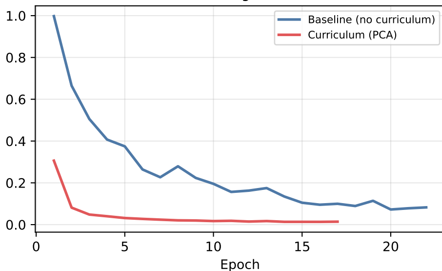
Validation V-Recall
