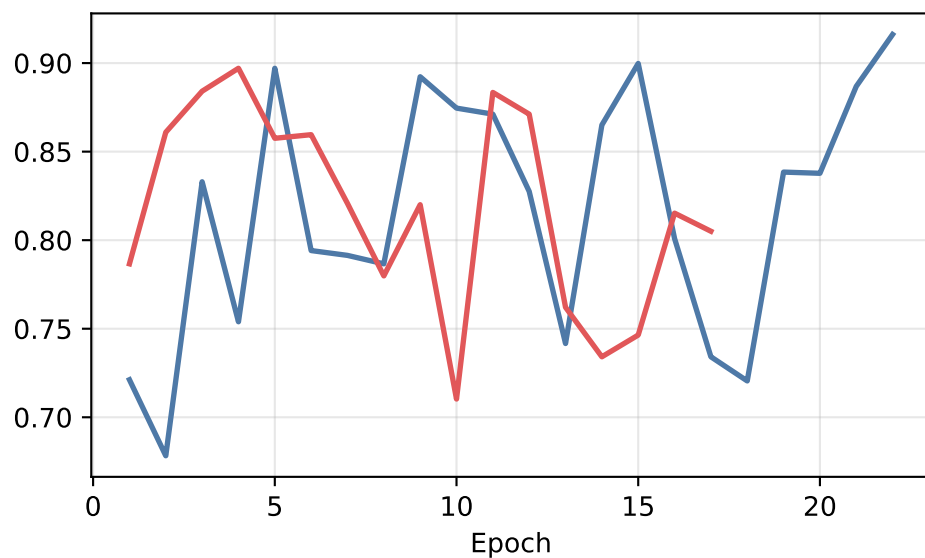
Validation V-Recall
