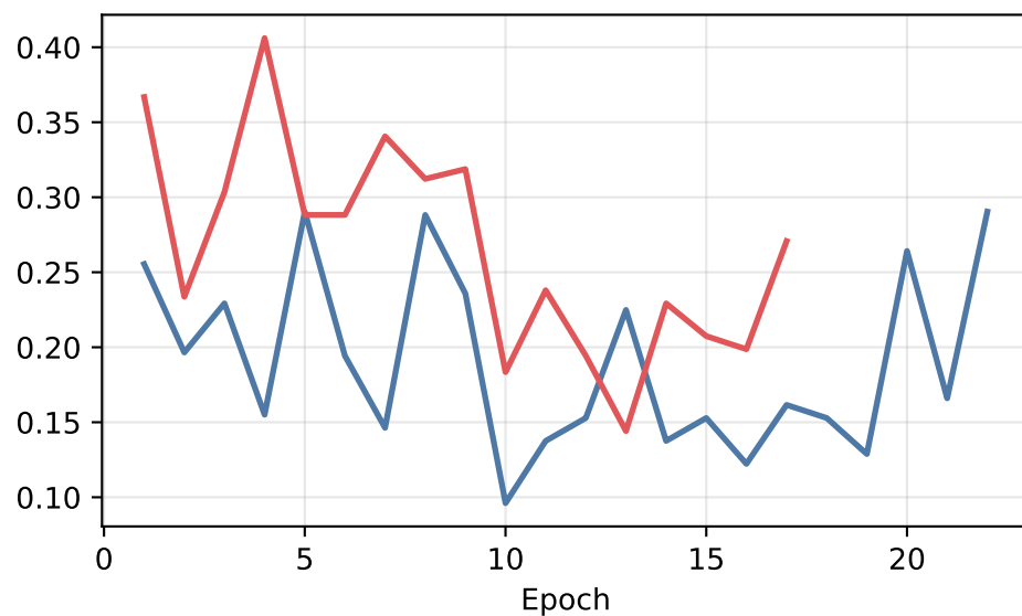
Validation S-Recall
