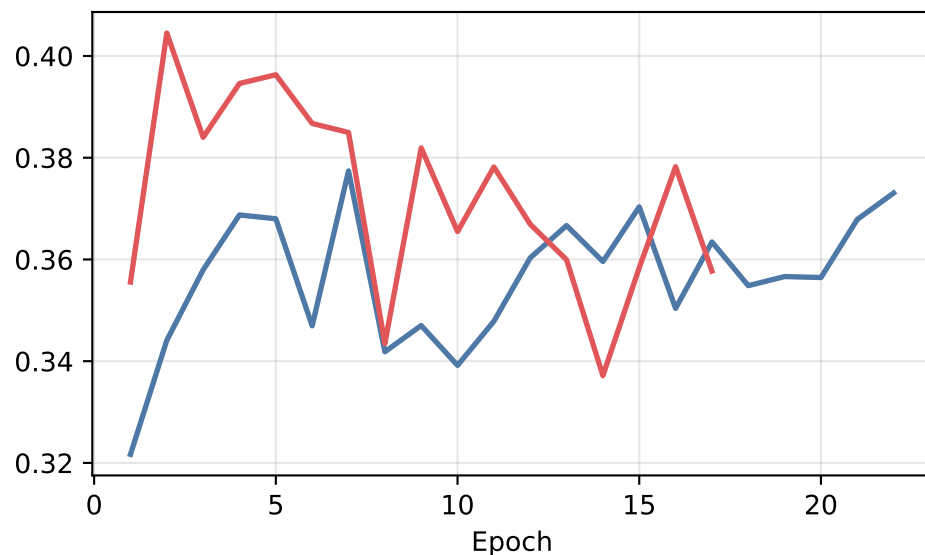
Validation S-Recall
