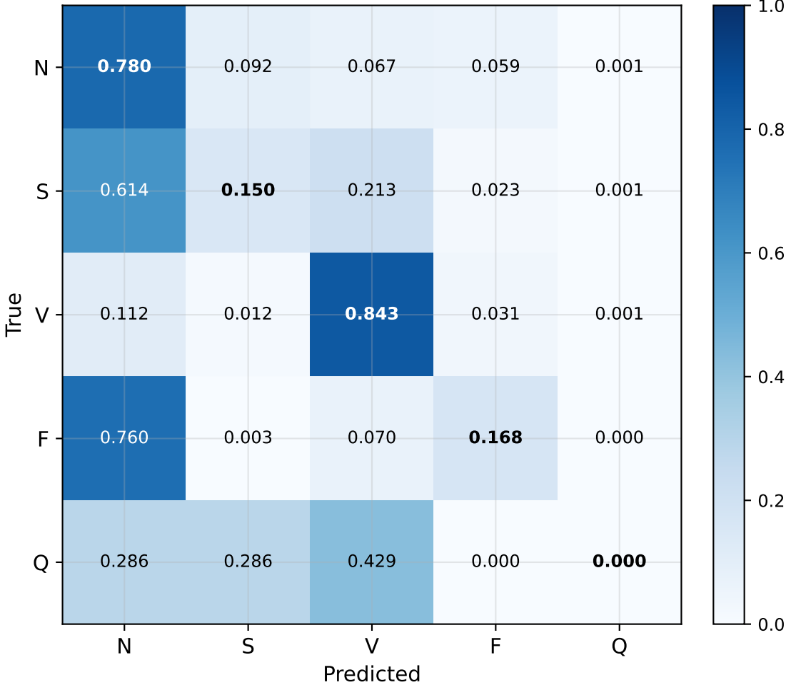
Normalised Confusion Matrix — WavKAN-v2 (DS2 Test Set, Seed 42)
