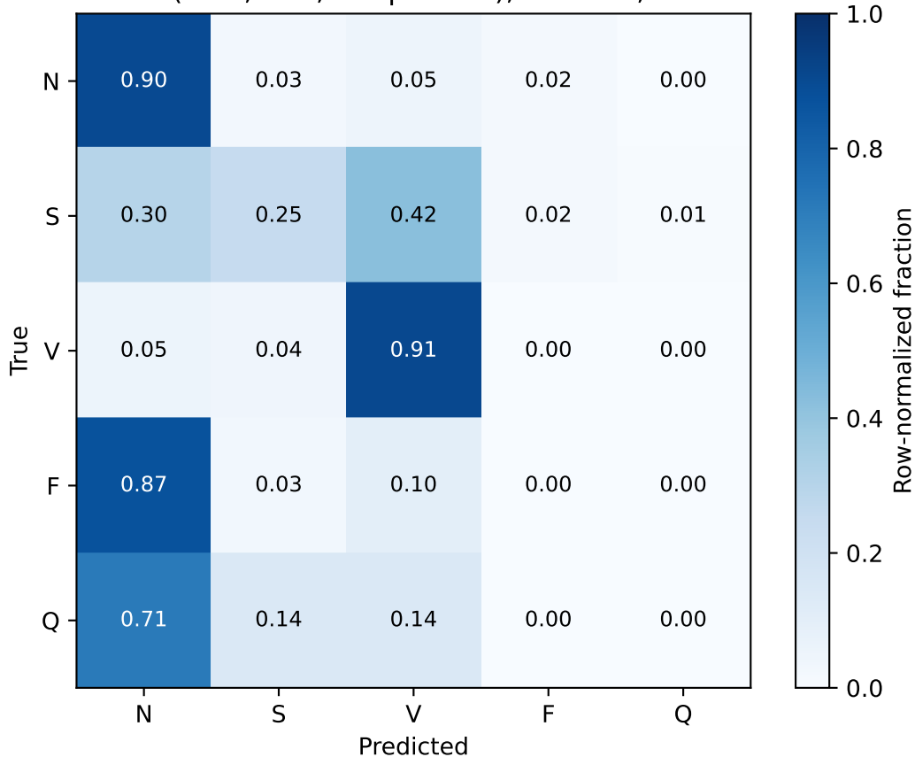
Normalized Confusion Matrix WavKAN-v2 (final, 153,045 params), seed 42, DS2 test set
