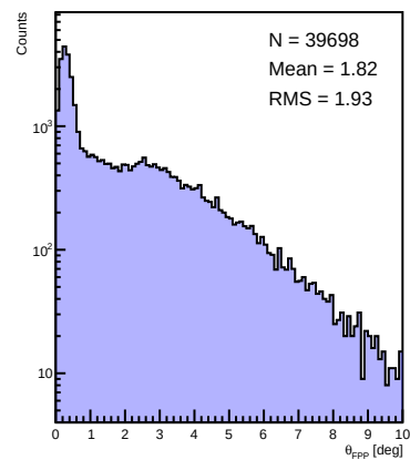
Before Alignment \theta_{\text{FPP}}
