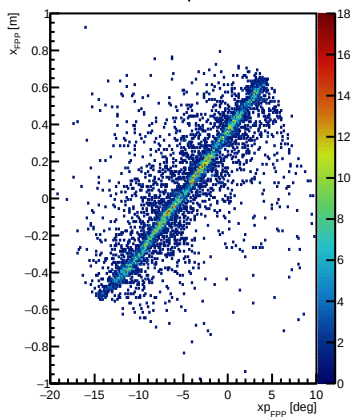
x vs x_P FPP
