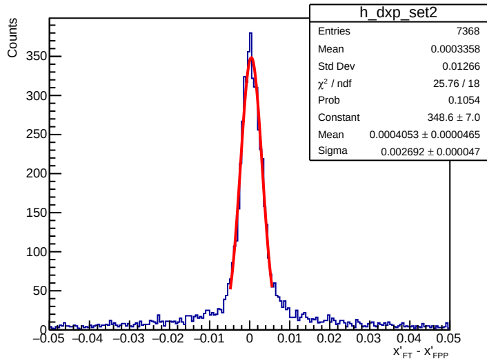
Track \Delta X'
