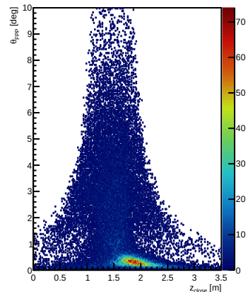
\theta_{\text{FPP}} vs z_{\text{close}}
