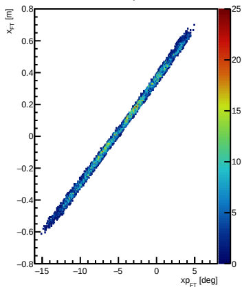
After Alignment x vs x_P FT
