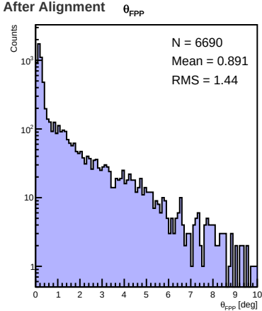
After Alignment
