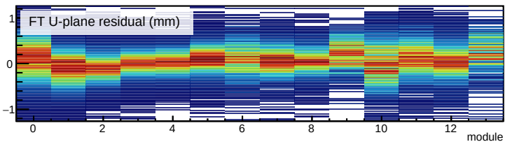
Before Alignment
