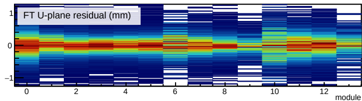
After Alignment
