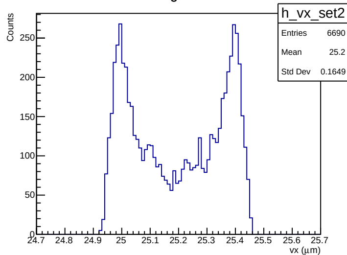
Target vx
