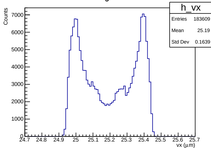
Target vx
