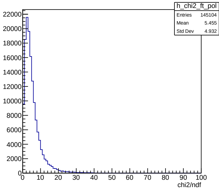
chi2/ndf FT
