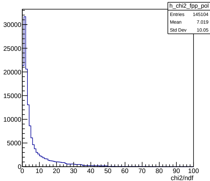
chi2/ndf FPP
