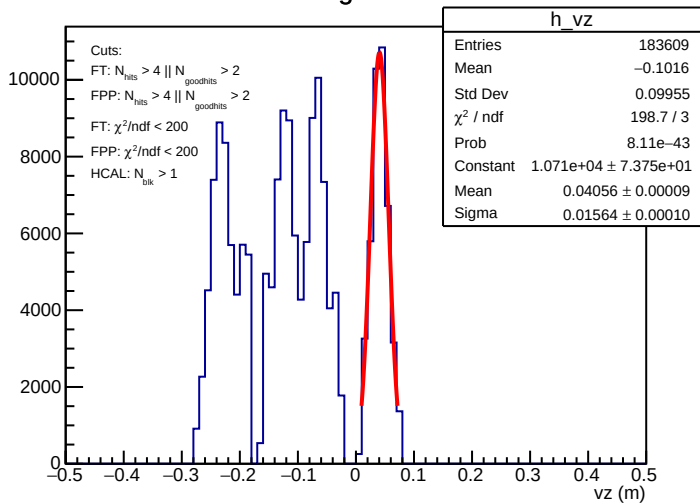
Target vz
