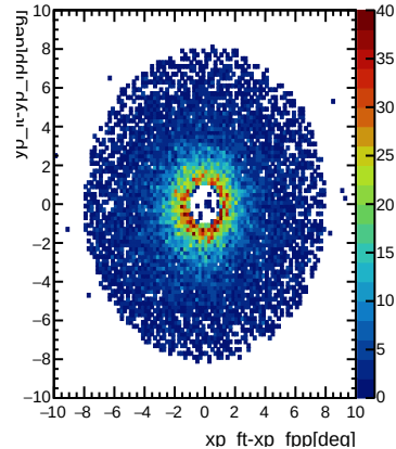
dpx vs dyp
